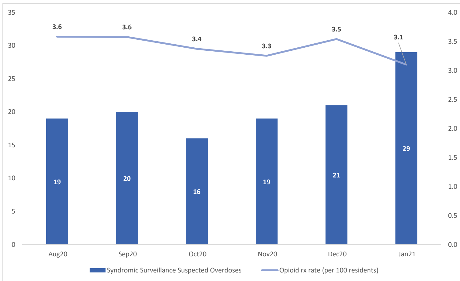
Figure 1. Suspected drug overdoses from Syndromic Surveillance and prescription (Rx) opioid rates (per 100 residents) in the Northern Region, August 2020 – January 2021
